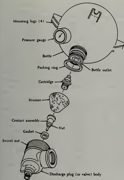
FIGURE 9-22. Components of a typical fire extinguisher container.
